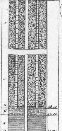
Sondage de Sidi Mached. Fig. 9.
