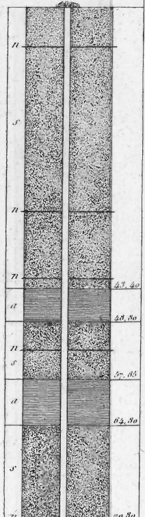
Sondage de Sidi Mached. Fig. 9.
